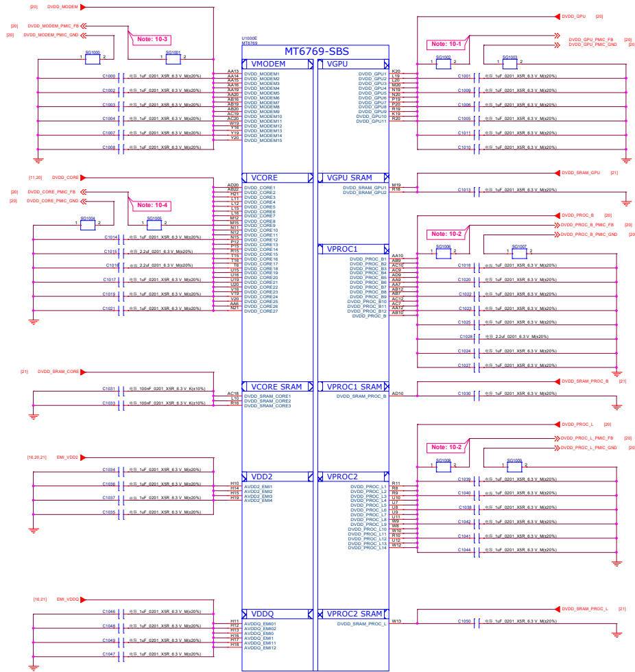
Schematic design notice of "10_BB_POWER_PDN" page:
